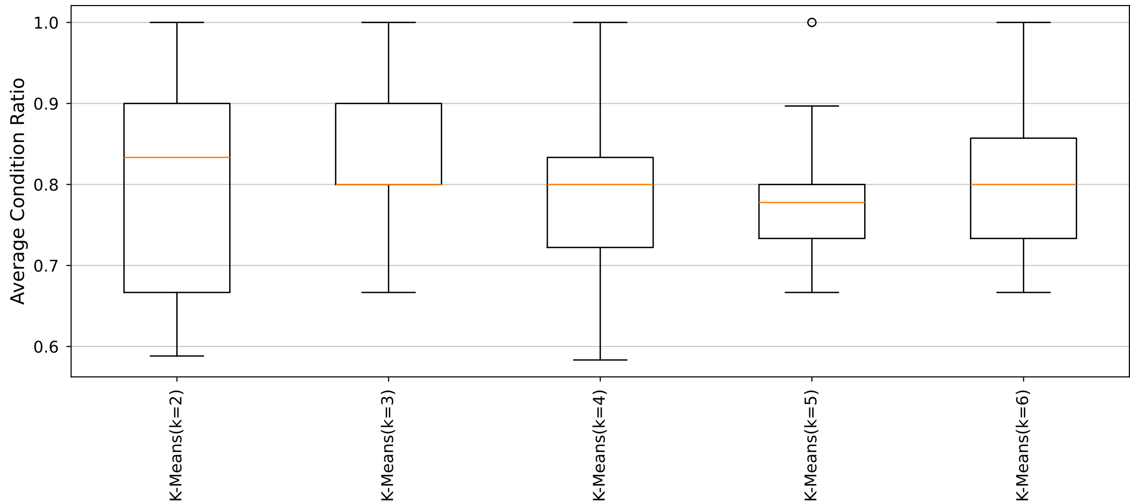
YARA Rules Average Condition Ratio Distribution (Cluster19_Size6 dataset)
